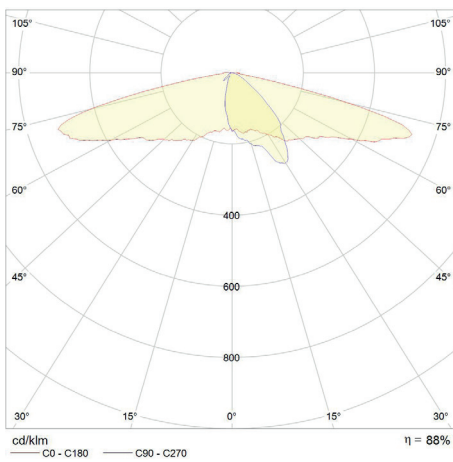
SAMSUNG LH502C
